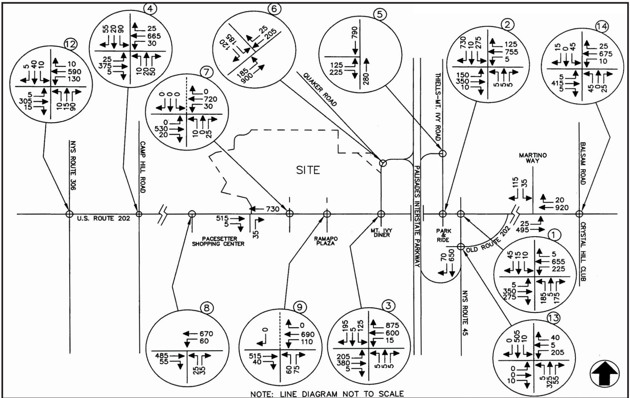
Figure 3.5-2: Existing Traffic Volumes Weekday Peak AM Highway Hour Minisceongo Park
